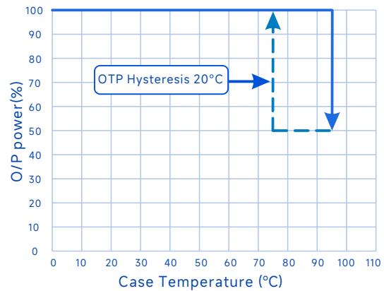
O/P Power Vs. Case Temperature (D model)
