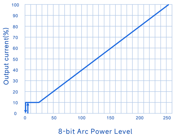
Linear Dimming Curve:(DMX Model)
